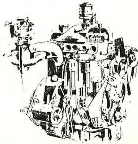
1939 O.H.V. (Pushrod) 1,100-c.c. Morgan (Standard) engine
